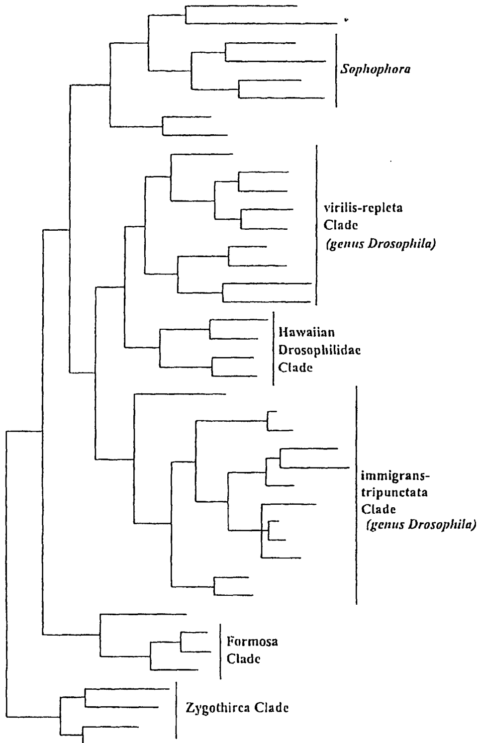
Figure 1. Phylogeny of the genus Drosophila and related groups showing the placement of the endemic Hawaiian Drosophila (Remsen & O'Grady, 2002). The Hawaiian Drosophila clade is nested within the genus Drosophila .
