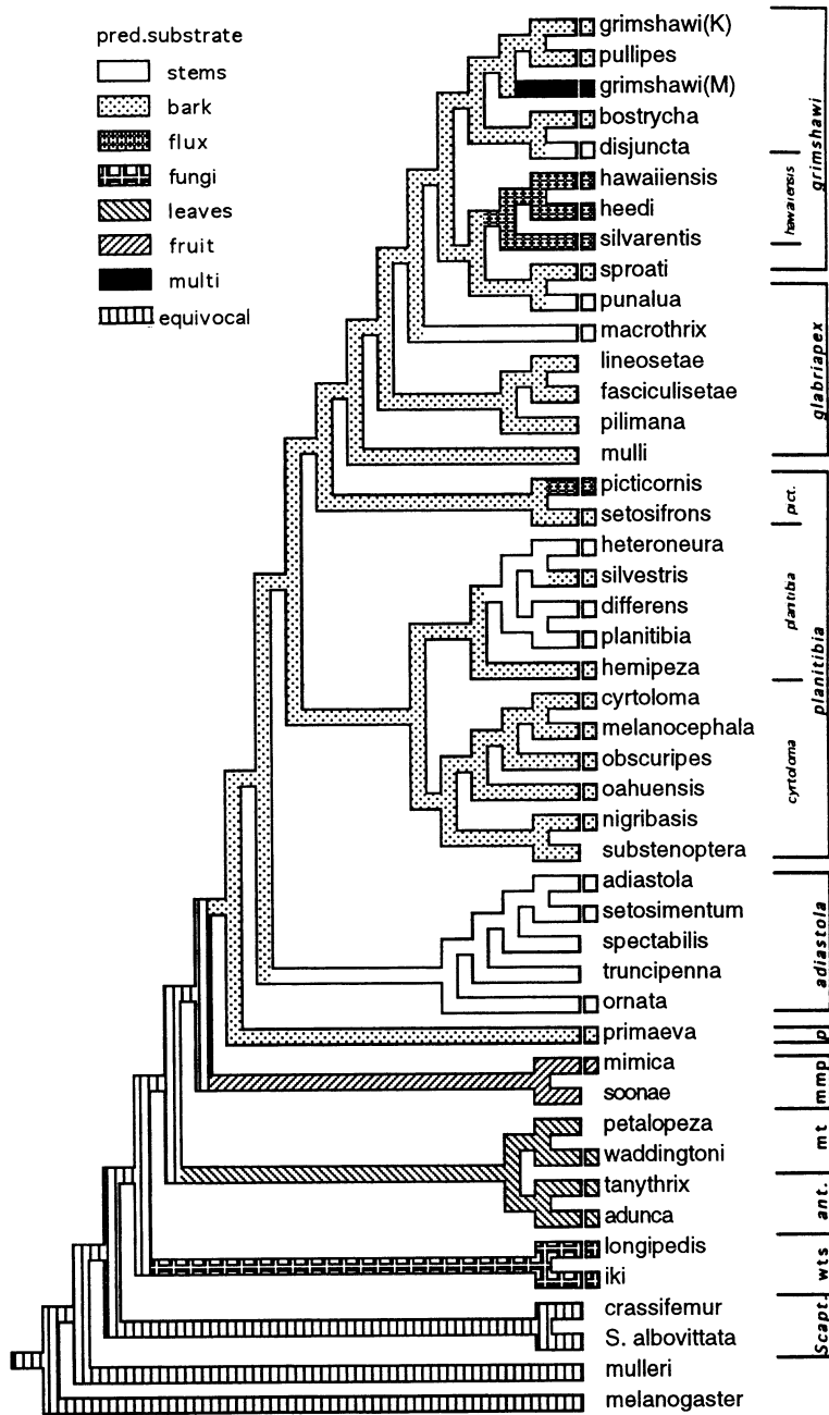
FIGURE 1. Pattern of ecological diversification in breeding substrates among the Hawaiian drosophilids. The character analyzed here is the predominant substrate used by each species for oviposition and larval development (see key and Materials and Methods). Phylogenetic character mapping on the molecular tree presented in Kambyseilis and Craddock (1997) was performed using the MacClade program (Maddison and Maddison 1992) with the accelerated transformation optimization implemented. The ecological data were taken from Heed (1968) and Montgomery (1975). Species for which no ecological data are available lack the small box at the end of the branch. Species are clustered into the formerly recognized species groups (in bold) and subgroups bracketed to the right of the tree. Reading from the bottom up abbreviations are as follows: Scapt. (the scaptomyzoid group); wts (white-tip scutellum group); ant. (antopocerus group); mt (modified-tarsi group); mmp (modified-mouthparts group); p ( primaeva species group—this and all the above species are included in the picture-wings); pict. (the picticornis subgroup of the planitibia species group). The K and M following D. grimshawi refer, respectively, to the Kaua'i and Maui populations, which recently have been recognized as distinct species. The Kaua'i population will be named as a new species (Kaneshiro, pers. comm.).
