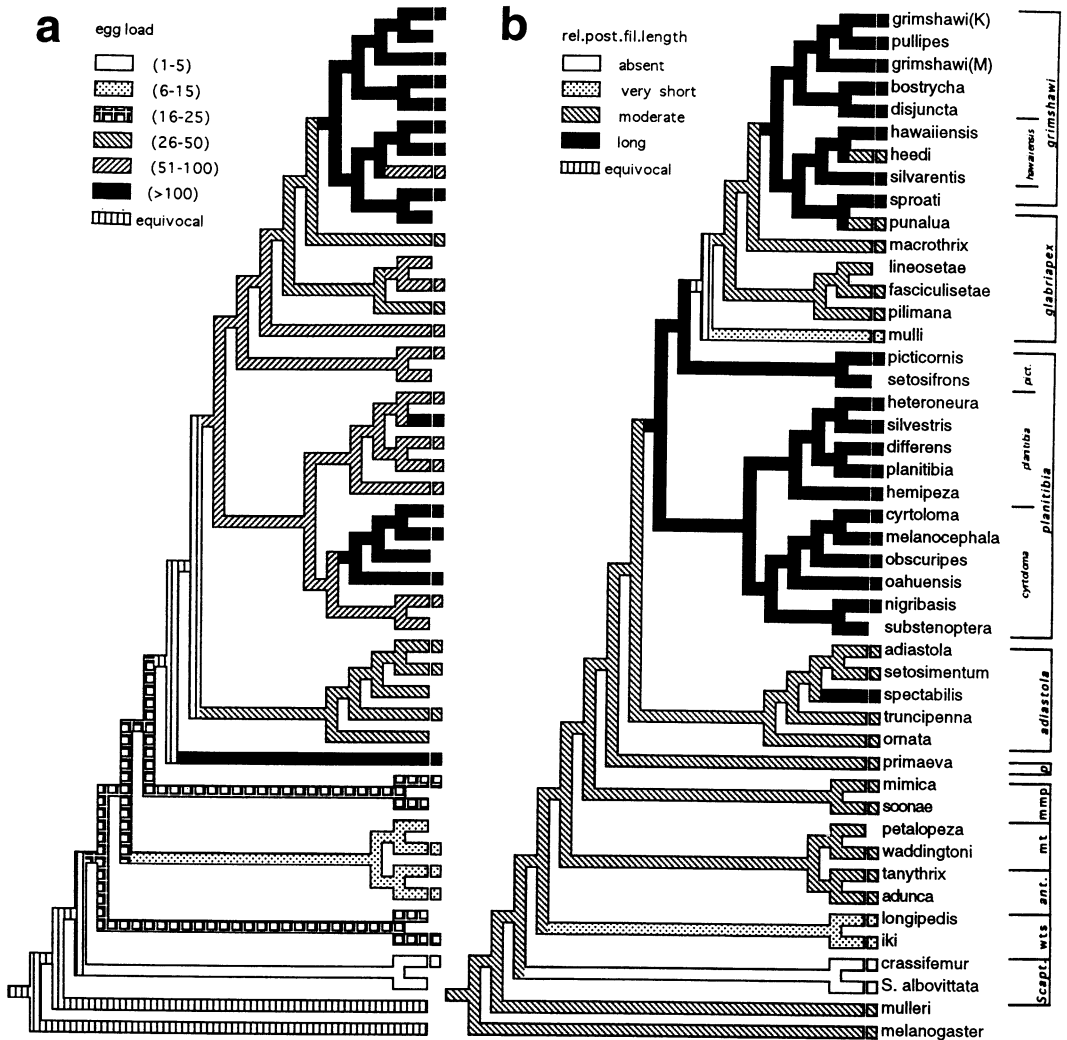
FIGURE 2. Phylogenetic pattern of evolution of two female reproductive traits among Hawaiian drosophilids. a . Egg load per fly; b . Length of the posterior respiratory filaments relative to the length of the egg (see keys and Materials and Methods for further details of the character classes). Data are from Kambysellis and Heed (1971) and unpubl. For both traits, the character reconstruction resulting from the accelerated transformation optimization (Maddison and Maddison 1992) is displayed.
