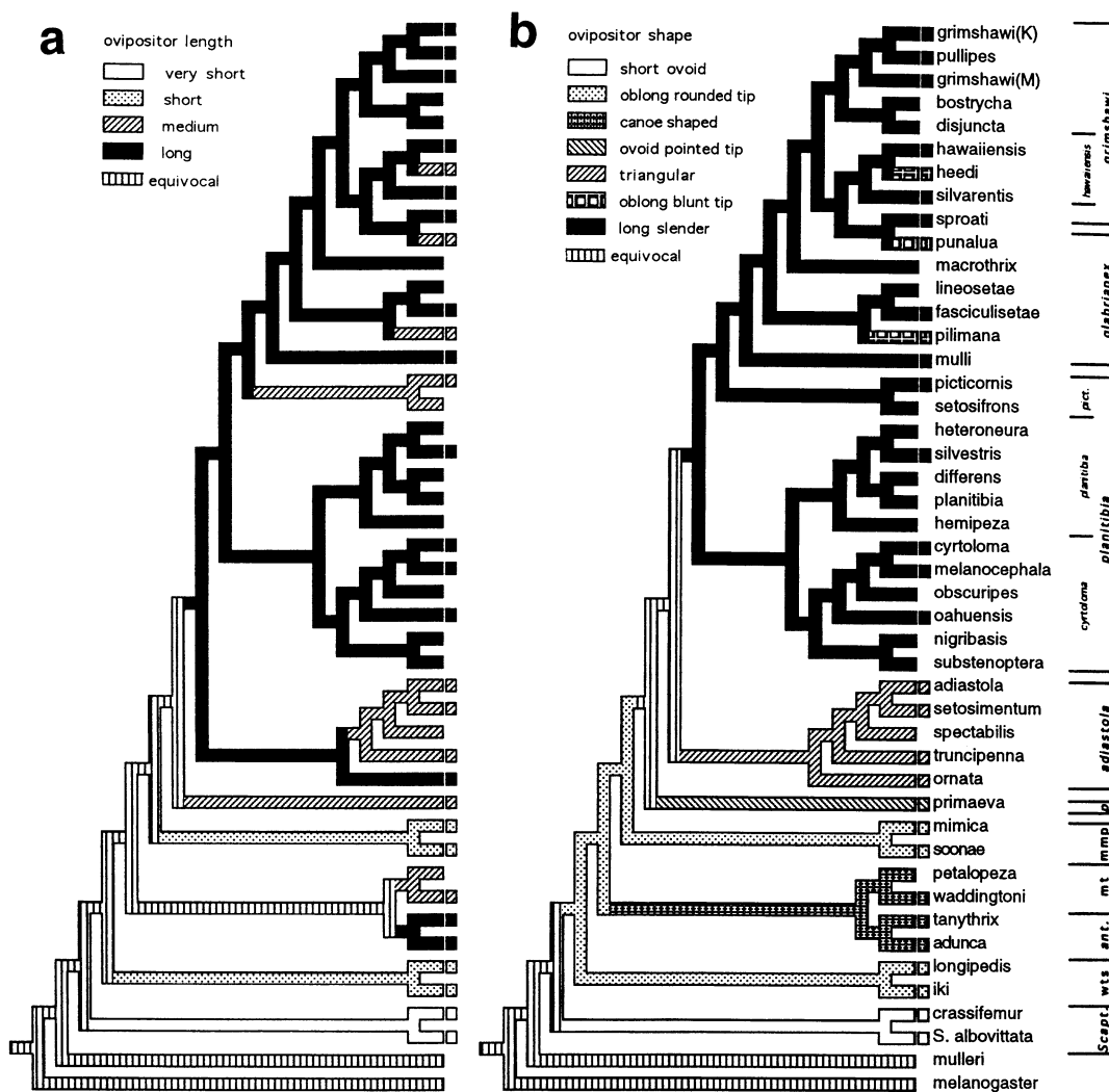
FIGURE 4. Evolutionary pattern of two ovipositor traits ( a , length, and b , shape) among Hawaiian drosophilids. Measurements were made from the scanning electron micrographs (see Figure 3, and text for coding of character states). For both traits, the accelerated optimization is displayed. In the case of ovipositor shape, the patterns from the parsimony reconstruction and the accelerated transformation optimization were identical.
